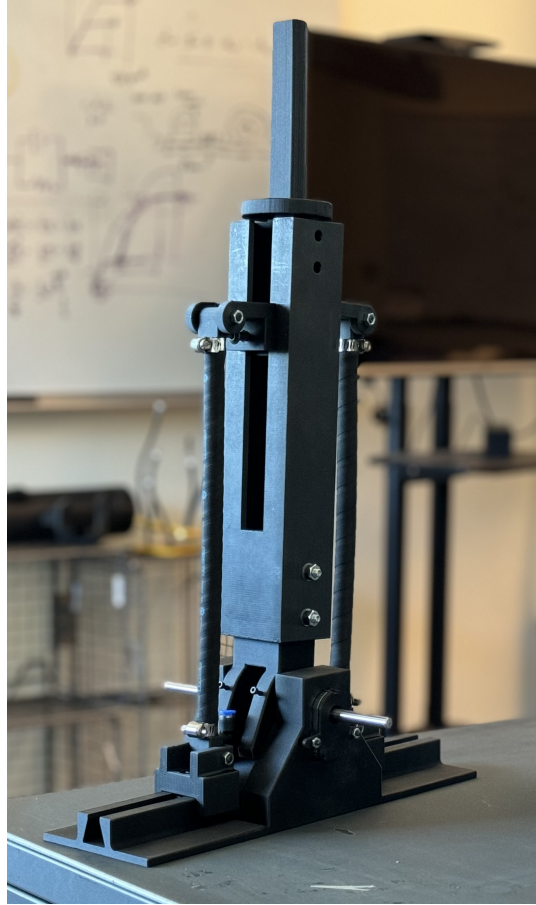
Figure 3.7: The BPA-actuated inverted-pendulum testbed. The pendulum shank rides on a hinge ankle above the foot assembly, and braided pneumatic actuators route down both sides of the shank to the foot, forming the antagonist ankle pair. Photograph from the AARL Inverted Pendulum project repository.
