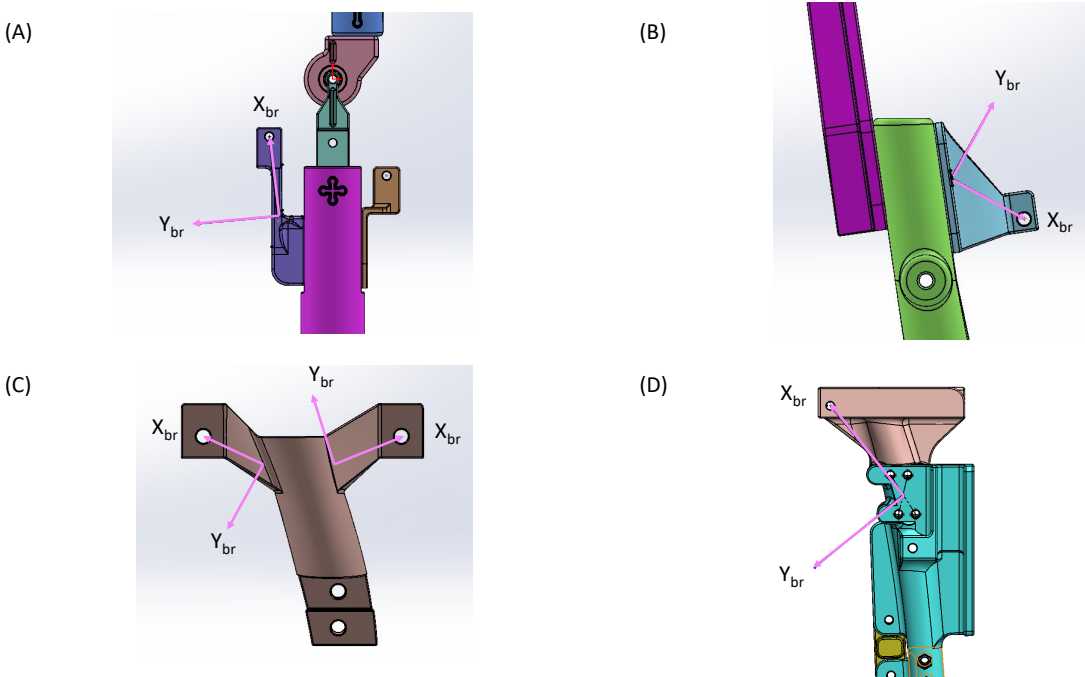
Figure 3.6: Bracket frame orientations for: (A) Flexor configuration on the pinned knee, (B) extensor configuration on the pinned knee, (C) flexor and extensor configurations on the biomimetic knee with \phi 10 mm BPAs, and (D) flexor configuration on the biomimetic knee with the \phi 20 mm BPA.
