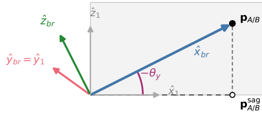
Figure 3.4: Two-rotation construction of the bracket frame from attachment point \mathbf{p}_A or \mathbf{p}_B . (A) Rotation through \theta_z about fixed \hat{z}_s aligns \hat{x}_1 with the point's sagittal-plane projection. (B) Rotation through -\theta_y about current \hat{y}_1 = \hat{y}_{br} aligns \hat{x}_{br} with the full point vector.
