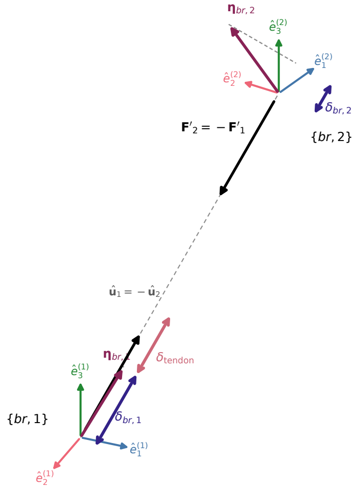
Figure 3.5: Two-bracket deflection and projection along the BPA force path. The force vectors at \{br, 1\} and \{br, 2\} point toward one another and satisfy \mathbf{F}'_2 = -\mathbf{F}'_1 . The bracket projections \delta_{br,1} and \delta_{br,2} are offset from the corresponding coordinate frames for clarity, and tendon elongation \delta_{tendon} continues collinearly from \delta_{br,1} . Colors follow a color-vision-deficiency-safe palette and are redundant with labels and line weights.
